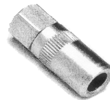
MANCHON DE RACCORD HYDRAULIQUE / GREASE GUN COUPLER * 1/8 X 27 NPT THREAD N° OU638025
