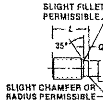
HALF DOG POINT
